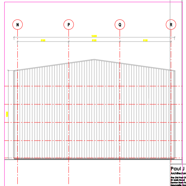
ELEVATION SOUTH - BLOCK 'J' AS PROPOSED
