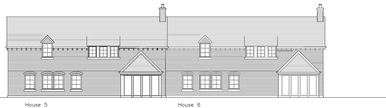
ELEVATION C
