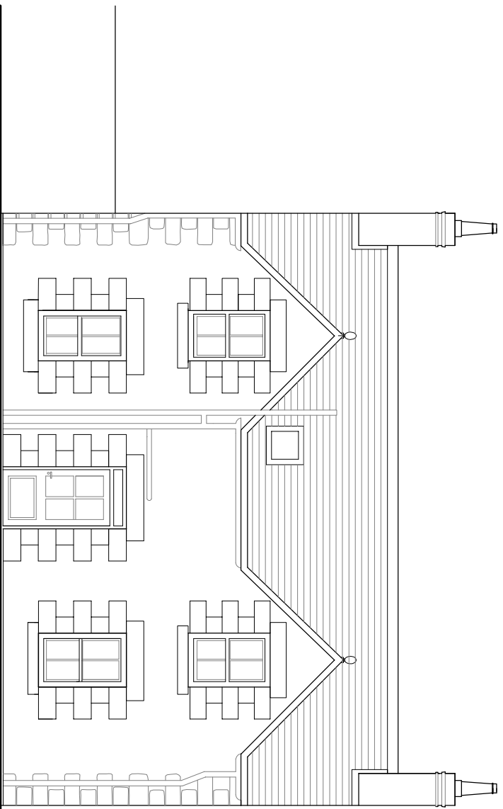
North Elevation
