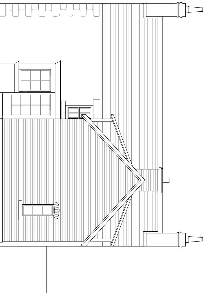
South Elevation
