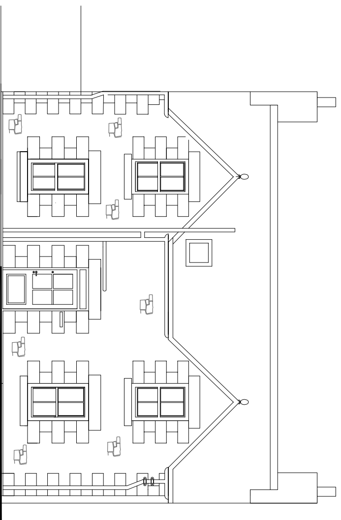
North Elevation
